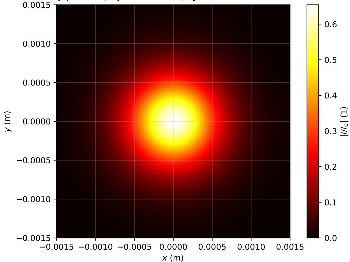
Intensity profile I(x, y, z = 3.821m)/I_0 , P_{in}=0.7P_{cr} , artificial time
